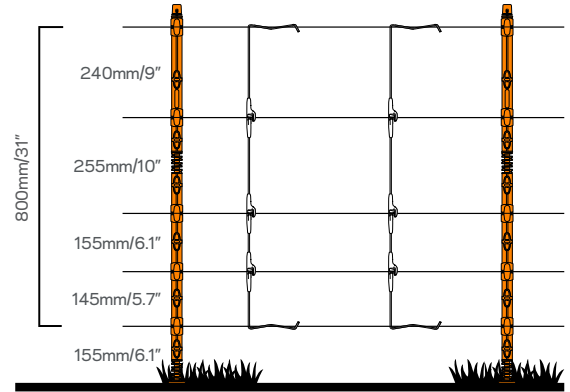
G71701 800mm/31" Electric Fence Dropper shown above
