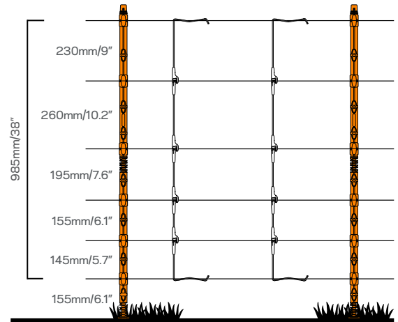
G71702 985mm/38" Electric Fence Dropper shown above
